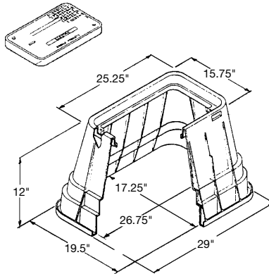
1324 Series Carson 12" Meter Box & Lid
