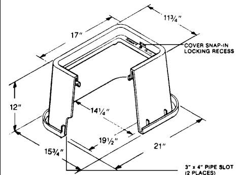
1419 Carson 12" Meter Box
